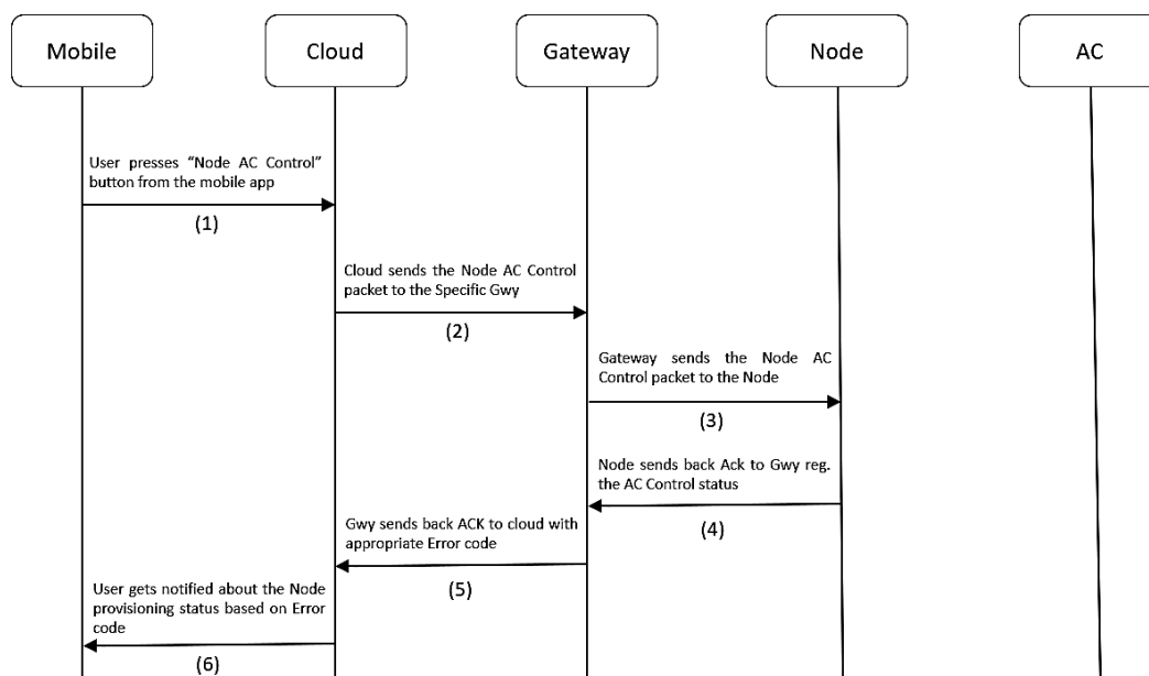
Figure 8.24 Node AC Control Process flow
