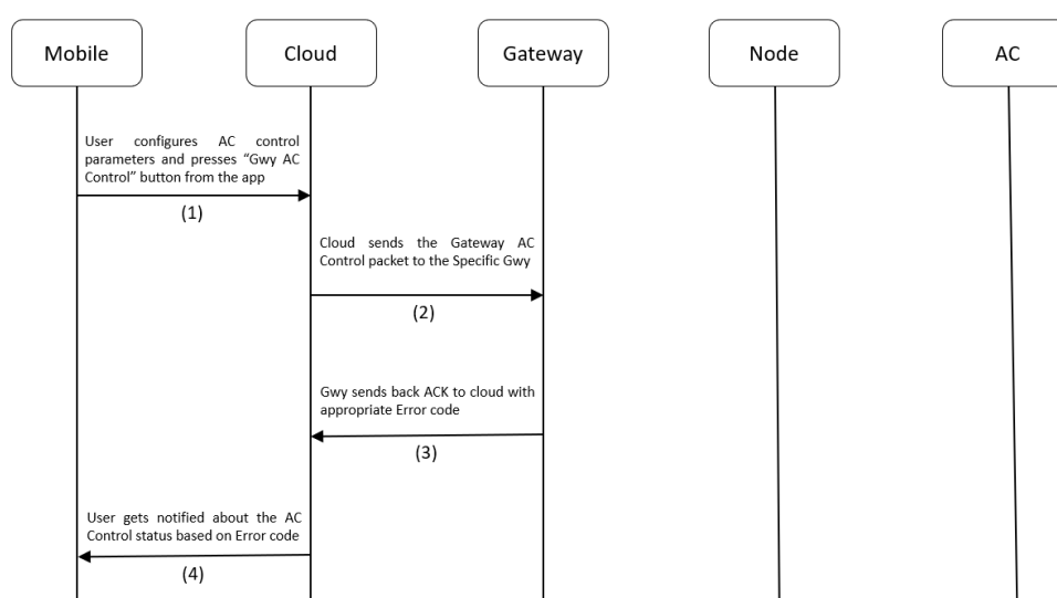
Figure 7 Gateway AC Control Process flow
